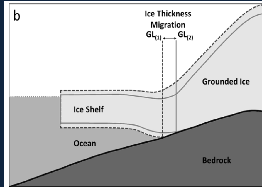
GL migration due to change in ice thickness
